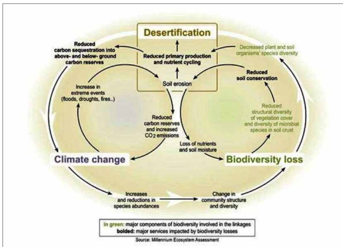
Figure 1. Generalised nexus between climate change, desertification and biodiversity loss
