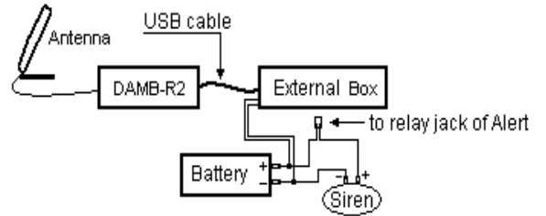
Figure 3: Components of the AREA Terminal device
