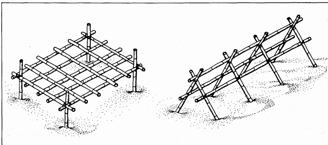
Fig. 8. Two methods of setting up intertidal lattice culture as used in the Philippines (after Ablan 1955).
