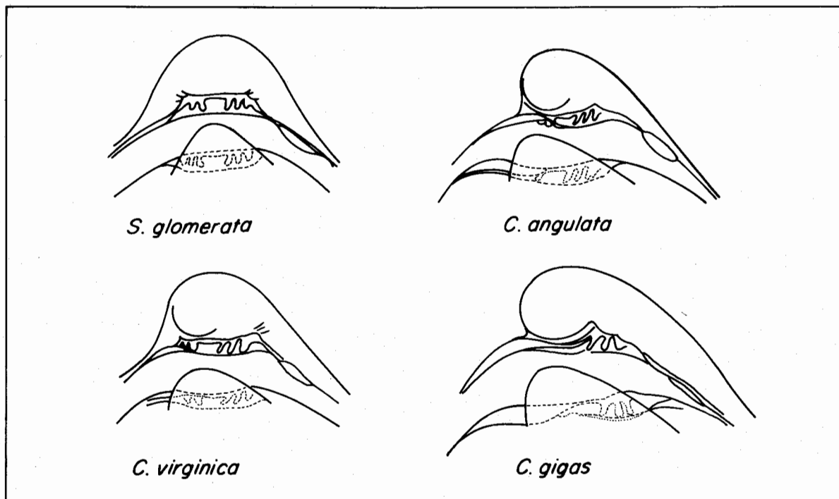
Fig. 1. Comparisons of the umbonal region of the prodissococonchs of four oyster species (after Dinamani 1976).
